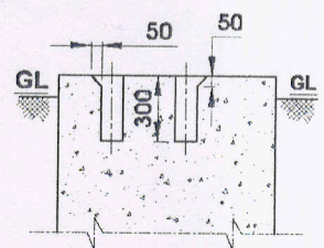
SECTION Z-Z
