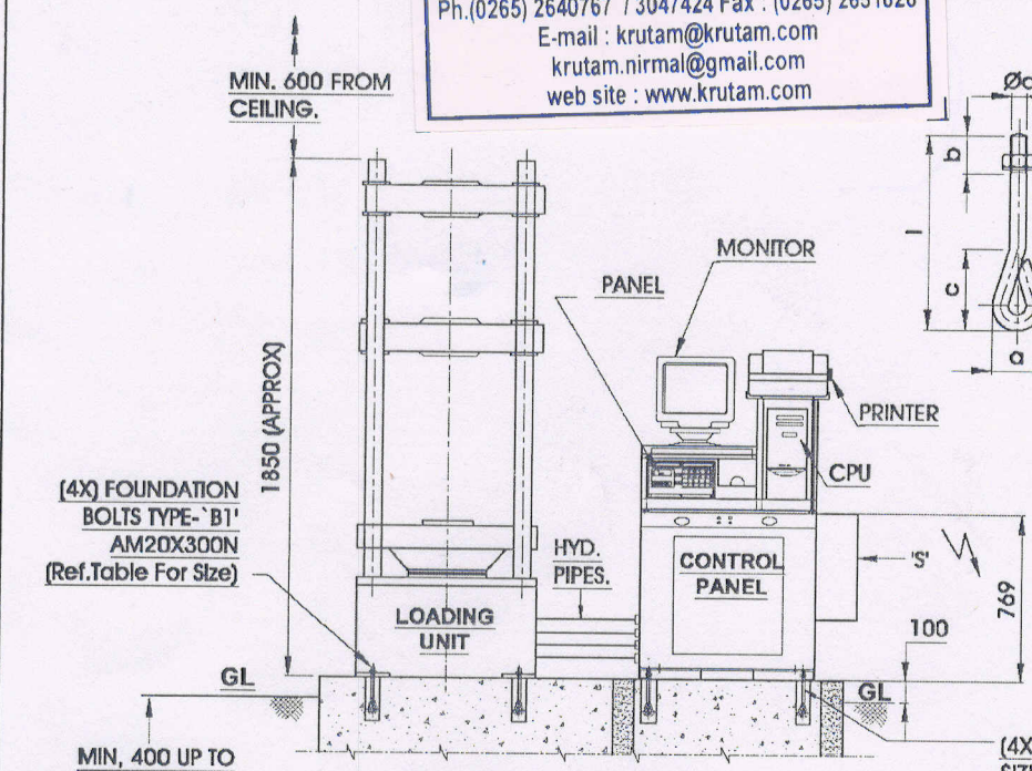
FRONT VIEW OF MACHINE
