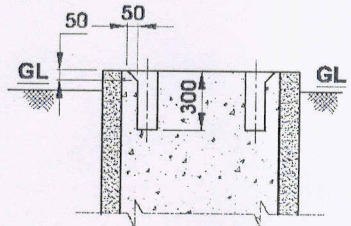
SECTION Y-Y
